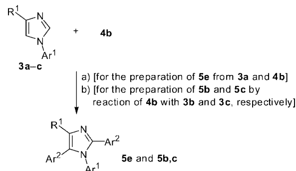
Scheme 4. Reaction conditions: a) 4b (2.0 equiv.), Pd(OAc) 2 (10 mol-%), Cs 2 CO 3 (2.0 equiv.), CuI (2.0 equiv.), DMF, 140 °C, 66 h, 32%. b) 4b (3.0 equiv.), Pd(OAc) 2 (10 mol-%), P( t Bu) 3 (20 mol-%) (for 3b ), [P( t Bu) 3 H] + BF 4 − (20 mol-%) (for 3c ), CsF (3.0 equiv.), CuI (3.0 equiv.), DMF, 140 °C, 114–281 h, 21% (for 5b ), 36% (for 5c ).
