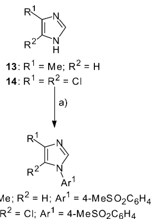
Scheme 3. Reaction conditions: a) NaH (1.03 equiv.), DMF, 0–20 °C, 2 h, then 4g (1.03 equiv.), DMF, room temp., 24 h (for 3f ) or 50 °C, 67 h (for 3g ), 75% for 3f , 78% for 3g .
