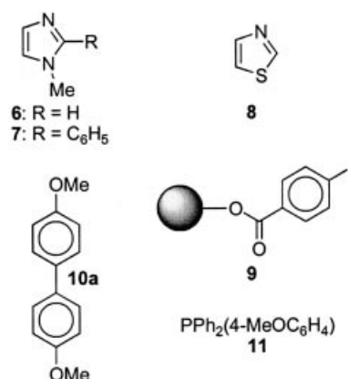
Figure 2. Chemical structures of compounds 6–9, 10a, 11.
