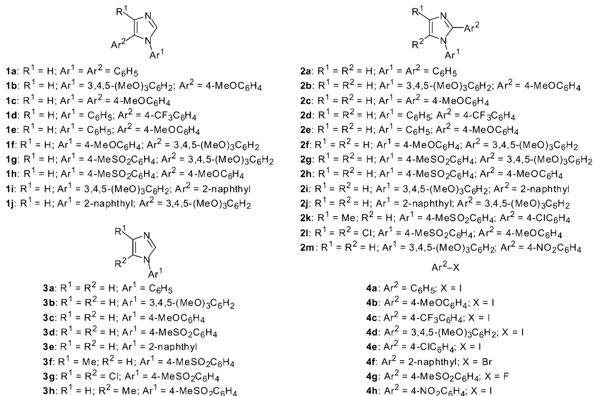
Figure 1. Chemical structures of compounds 1–4.
