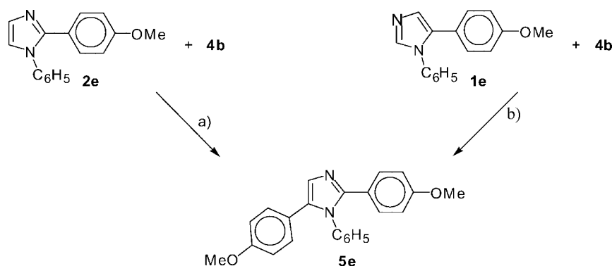
Scheme 5. a) 4b (2.0 equiv.), Pd(OAc) 2 (5 mol-%), CsF (2.0 equiv.), CuI (2.0 equiv.), DMF, 140 °C, 113 h, 57% (GLC). b) 4b (2.0 equiv.), Pd(OAc) 2 (5 mol-%), CsF (2.0 equiv.), CuI (2.0 equiv.), DMF, 140 °C, 46 h, 74% (GLC).
