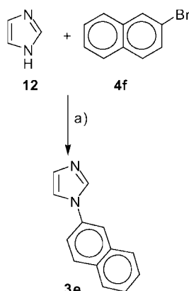
Scheme 2. Reaction conditions: a) 12 (1.5 equiv.), (\text{CuOTf})_2 -toluene (5 mol-%), dba (5 mol-%), 1,10-phenanthroline (1.0 equiv.), \text{Cs}_2\text{CO}_3 (1.1 equiv.), xylenes, 110 °C, 71 h, 61 %.
